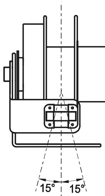
Fig. 2.2 Cable Deflection with Roller
